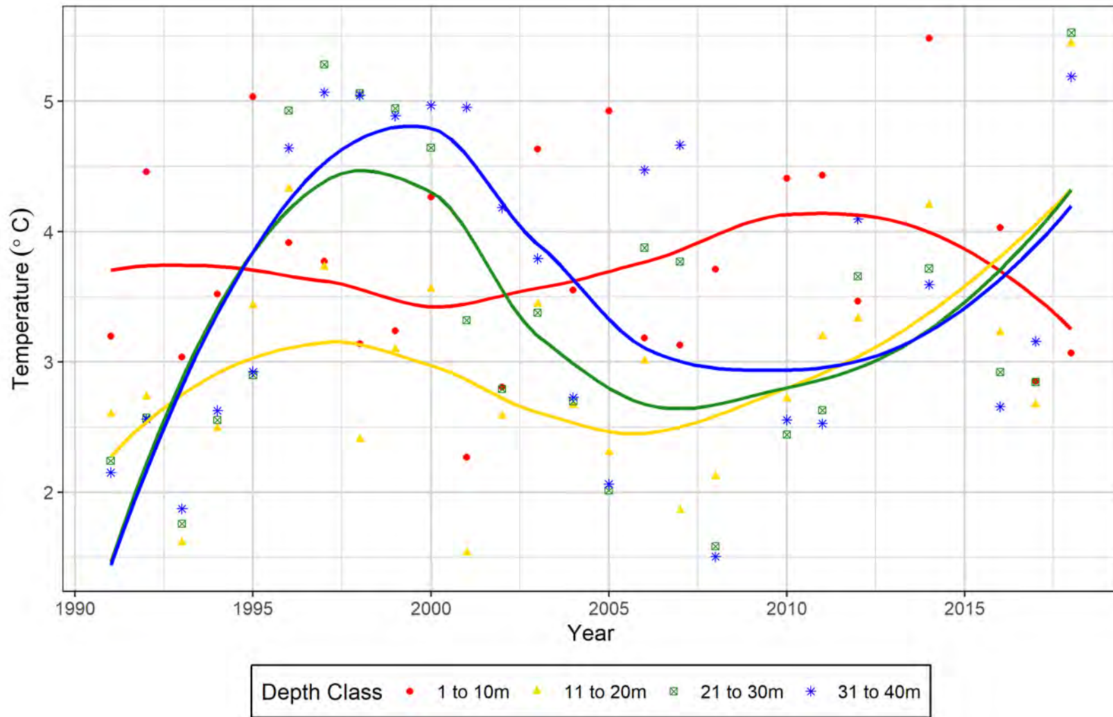
Figure 3.2-52. Average Water Temperature at 4 Depth Classes in Spring at Station 6
