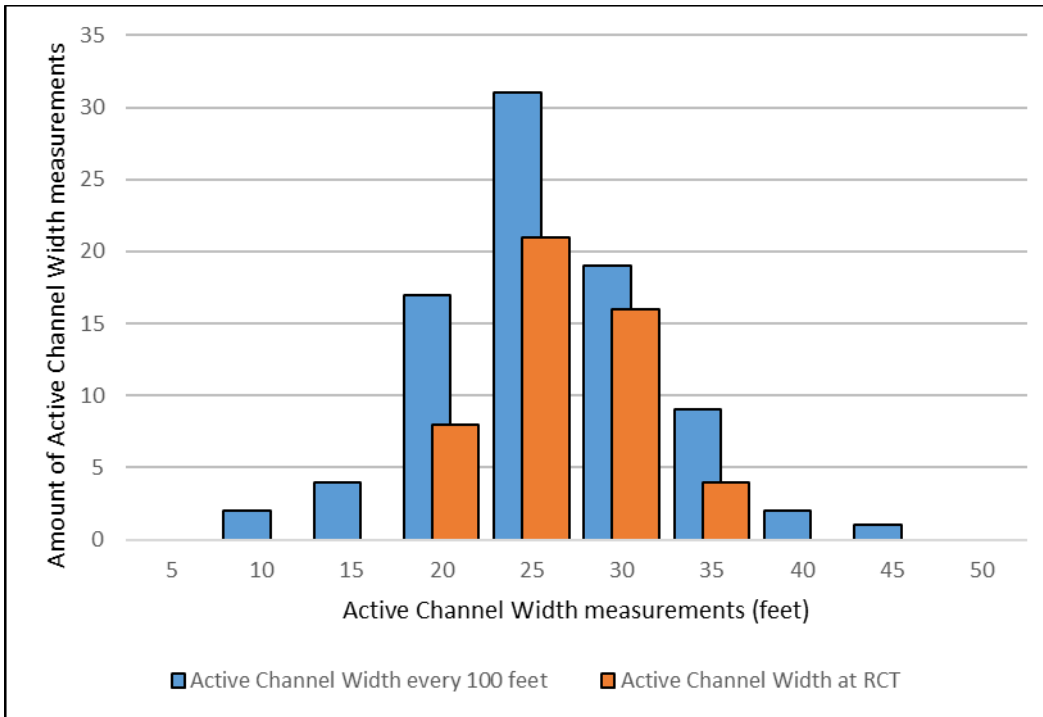
Figure 11. Distribution of active channel widths measured at riffle crests (orange) and every 100 feet (blue) for the upper and lower reach. Each measurement was grouped in increments of five feet (e.g., the '20' on the X axis includes recorded values ranging from 20.00 feet to 24.99 feet).
