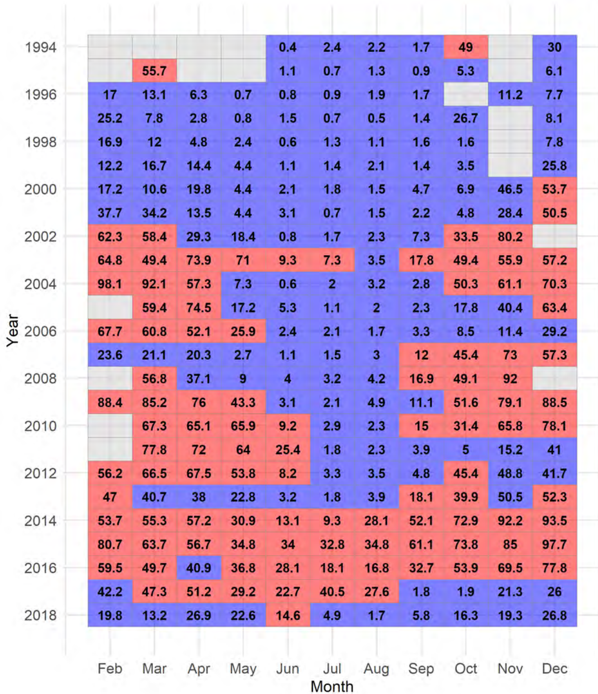
Figure 3.2-29. Average Chlorophyll a ( \mu\text{g/L} ) at Station 6 between 1 and 10 m Red colored cells indicate above the long-term average of the respective month while blue colored cells indicate below the long-term average of the respective month.
